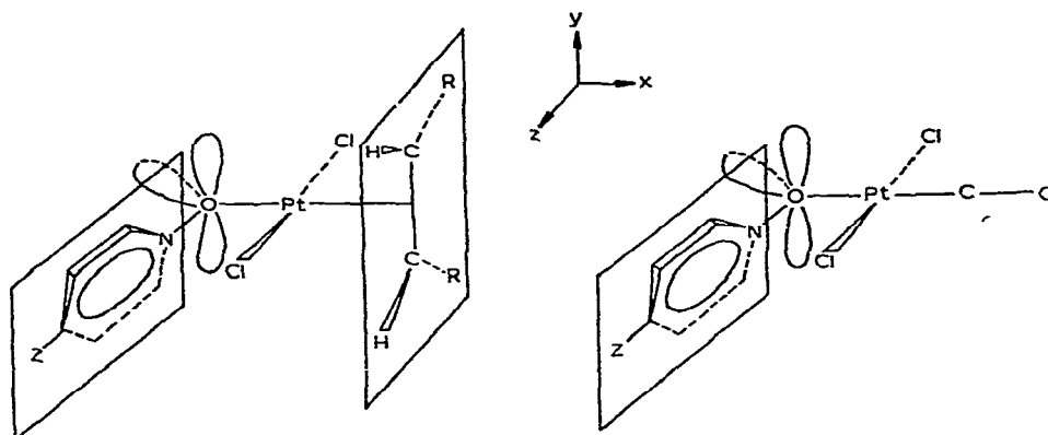
Fig. 2. Olefin and carbonyl complexes, 1 ( \text{L} \approx \text{olefin, CO} ).
