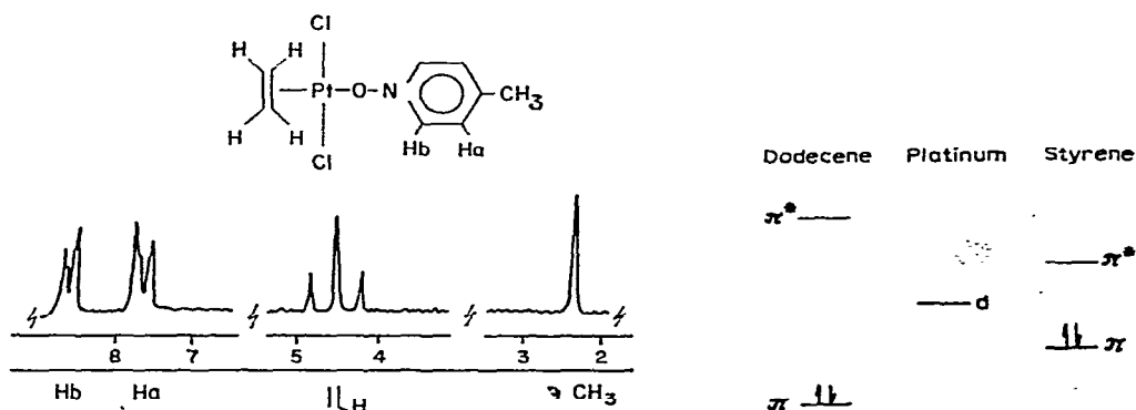
Fig. 8. NMR Spectrum of PyO complex 1 in \text{DCCl}_3 (L, \text{C}_2\text{H}_4 ; Z, \text{CH}_3 ).
